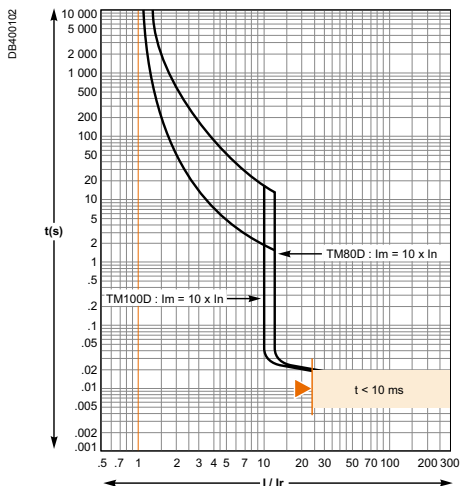
Reflex tripping.
